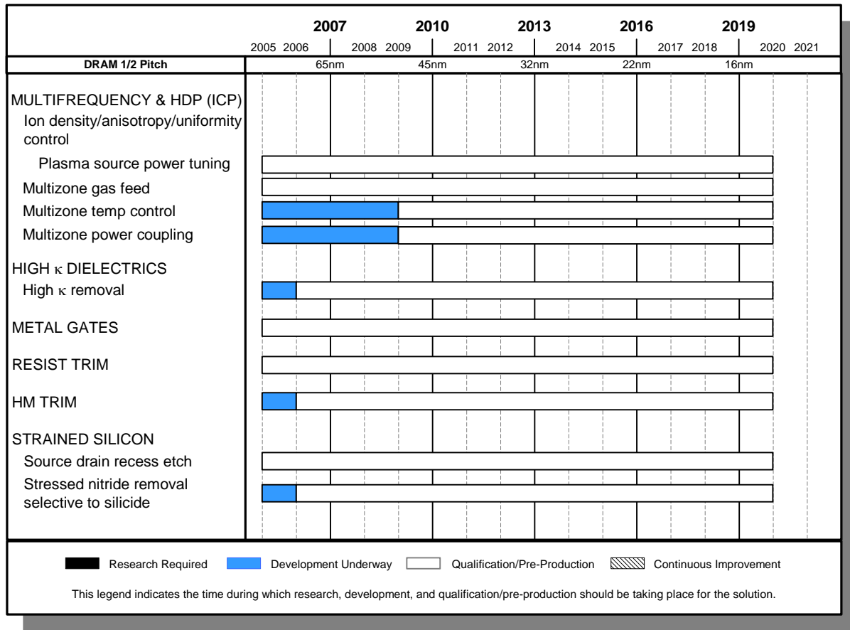
Figure 60 Front End Processes Etching Potential Solutions
